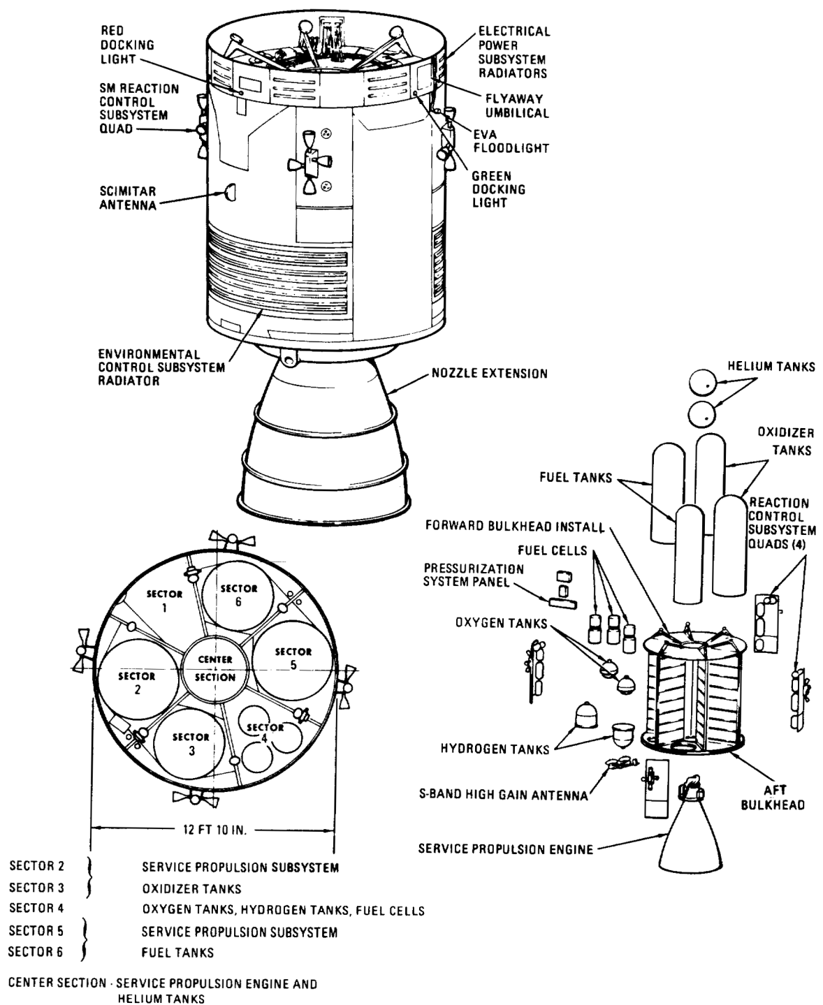
Figure 3-6.- Service module.
